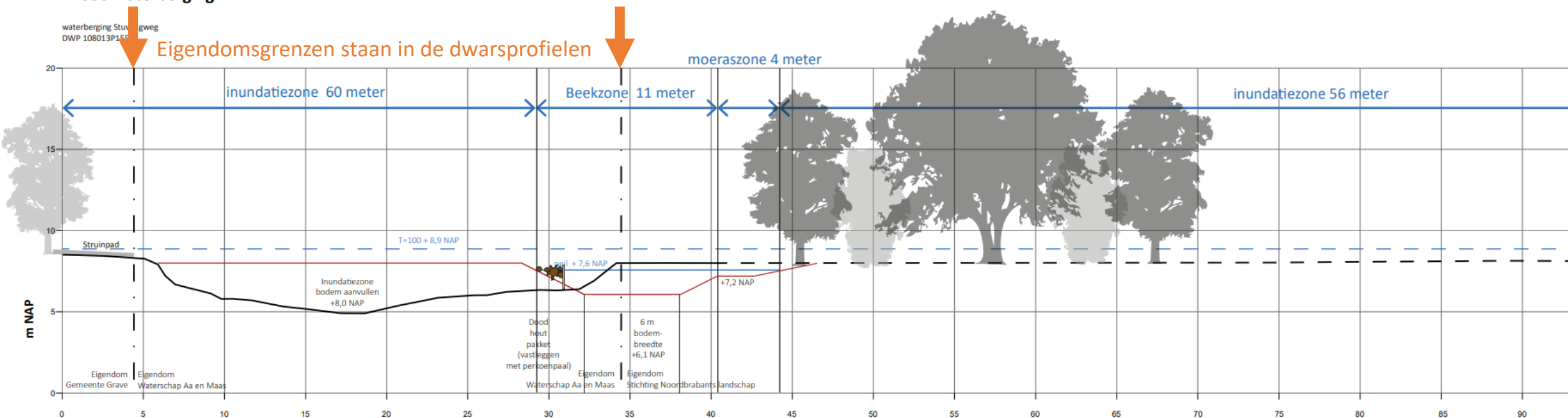
Profiel 1-3 P1550 waterberging
